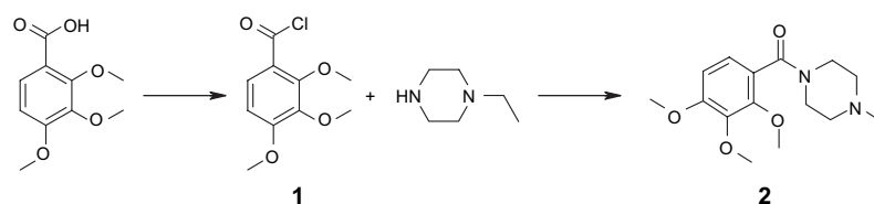
Fig. 6. SP008 chemical synthesis.
