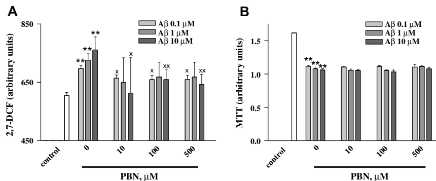
Fig. 4. Effect of the anti-oxidant phenyl- tert -butylnitron (PBN) on the A\beta_{1-42} -induced free radical production and cell viability on PC12 cells. PC12 cells were pre-incubated for 24 h with increasing concentrations of PBN before being exposed to increasing concentrations of A\beta_{1-42} . Free radical production was measured using the fluorescent probe 2,7-DCF (A) and cell viability assessed using the MTT assay (B) after 24 h of A\beta_{1-42} exposure. Control cells were exposed to vehicle only. Statistical analysis was performed using one-way ANOVA followed by Dunnett's test. Data shown are means \pm SD, n=6 , compared to the respective 0 \mu M group. ** p<0.01 compared to the control. ^x p<0.05 , ^{xx} p<0.01 compared to 0 \mu M.
